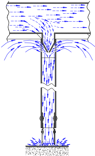
Typical Downspout
